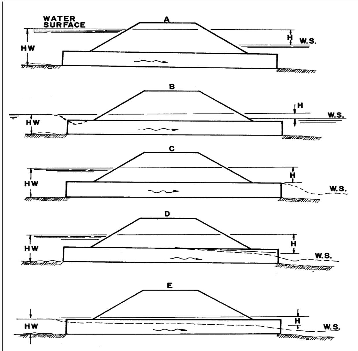
Figure 8-2: Five Outlet Control Conditions
